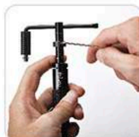
2. Set-up locking block to adjust coil insert depth
