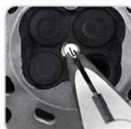
5. Using Pliers, take off pin on insert
